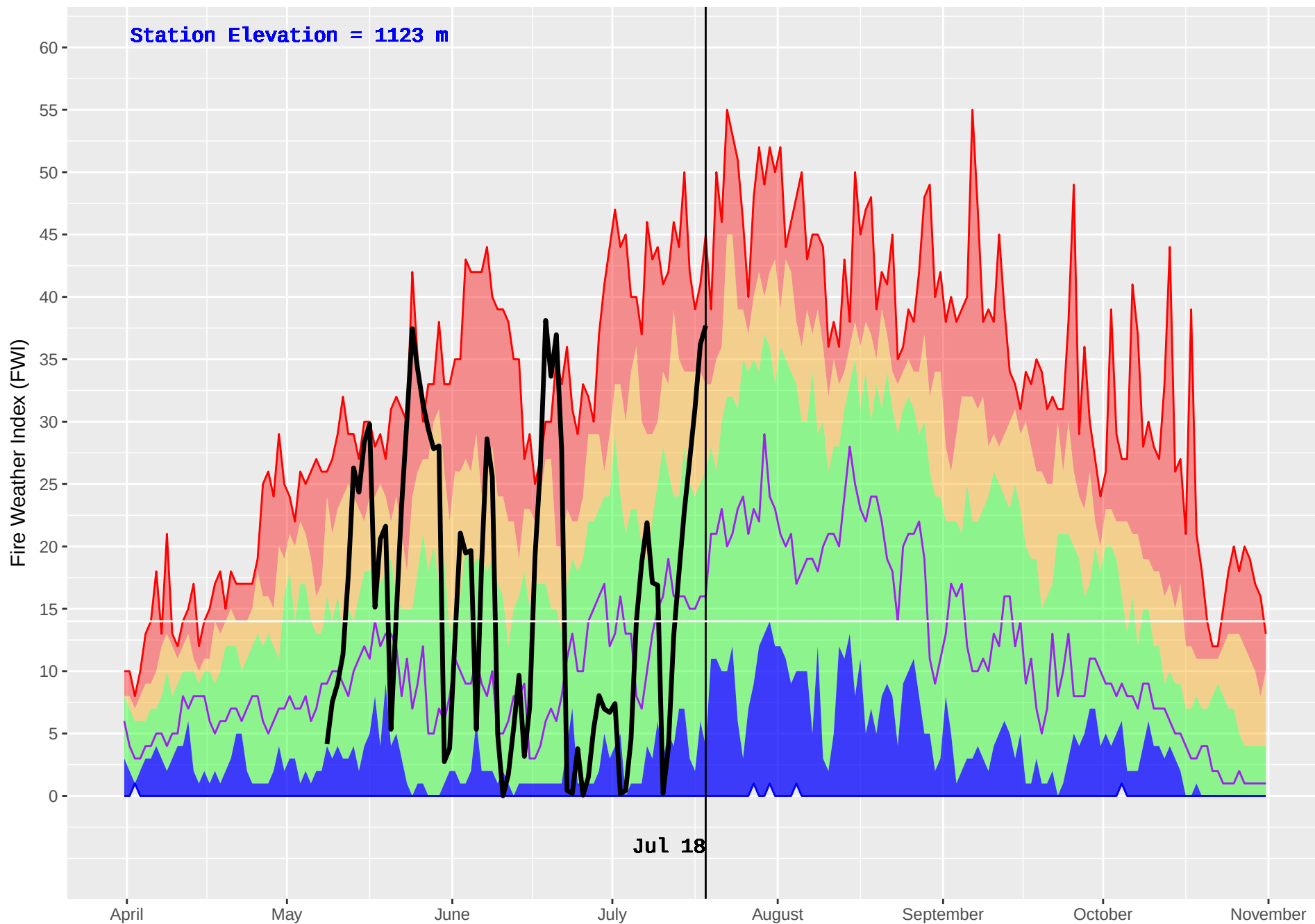
MCLEAN LAKE (311) : Historical (1987–2016) and Current (2018) Daily Fire Weather Index (FWI)
