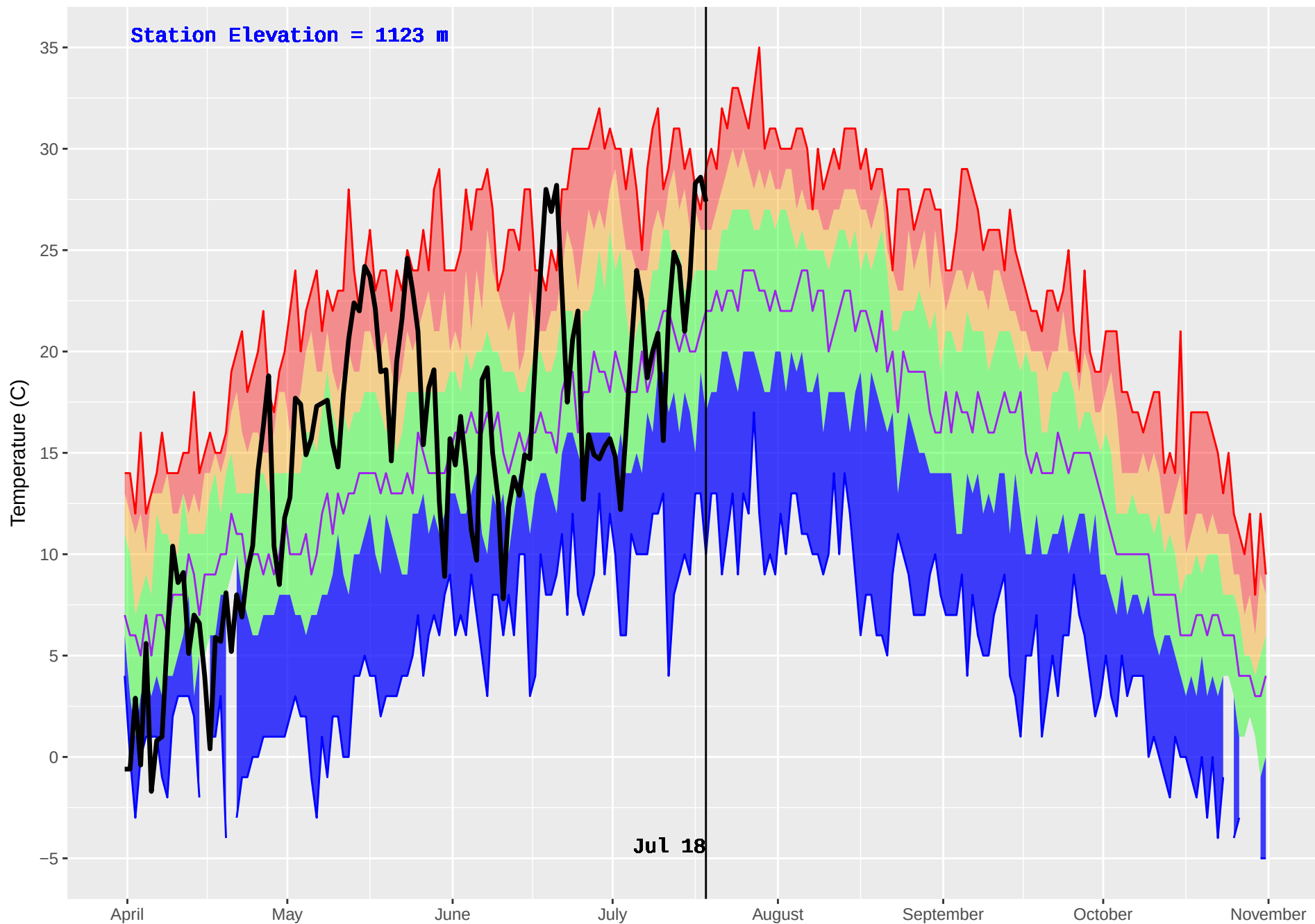
MCLEAN LAKE (311) : Historical (1987–2016) and Current (2018) Daily Temperature
