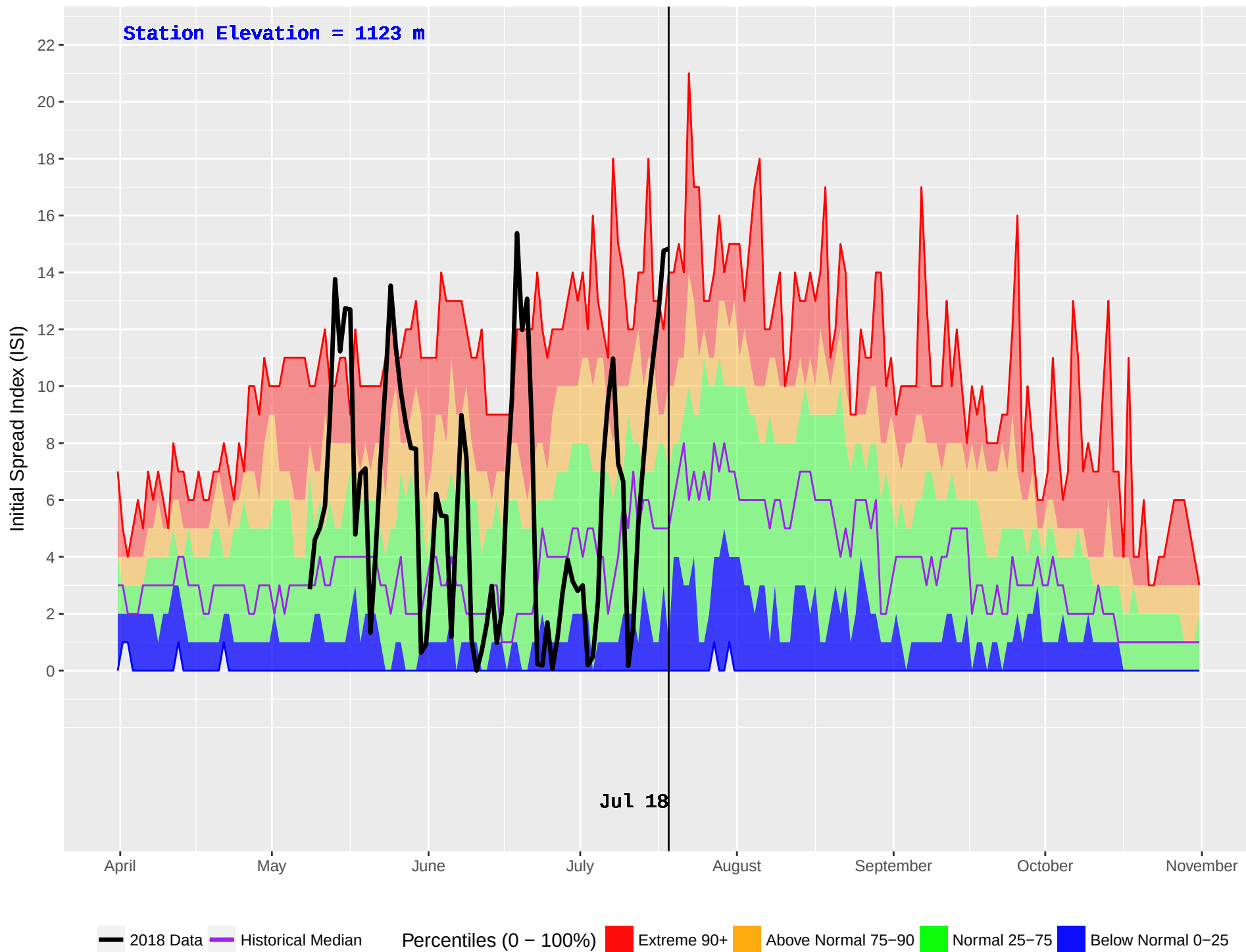
MCLEAN LAKE (311) : Historical (1987–2016) and Current (2018) Daily Initial Spread Index (ISI)
