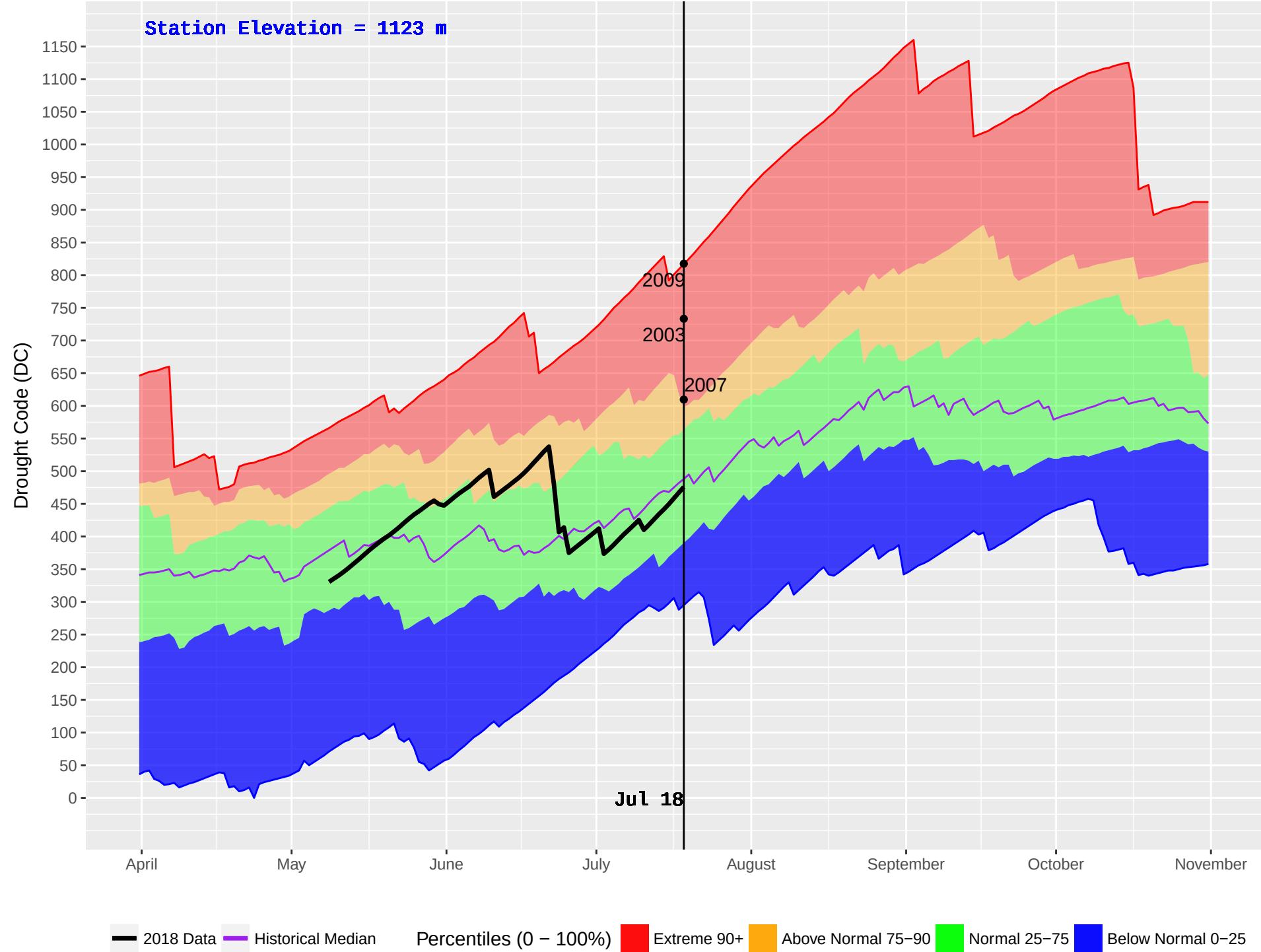
MCLEAN LAKE (311) : Historical (1987–2016) and Current (2018) Daily Drought Code (DC)
