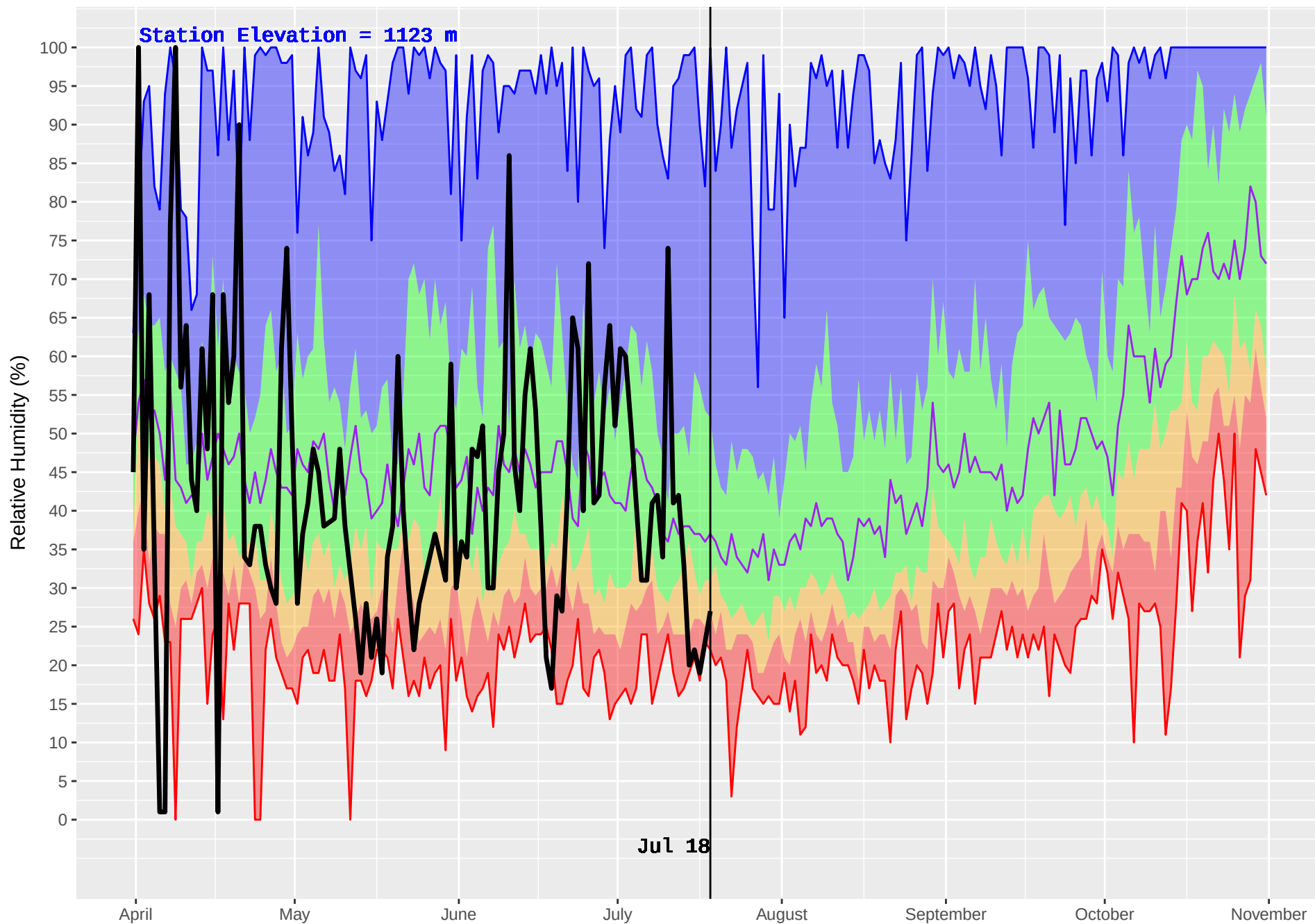
MCLEAN LAKE (311) : Historical (1987–2016) and Current (2018) Daily Relative Humidity
