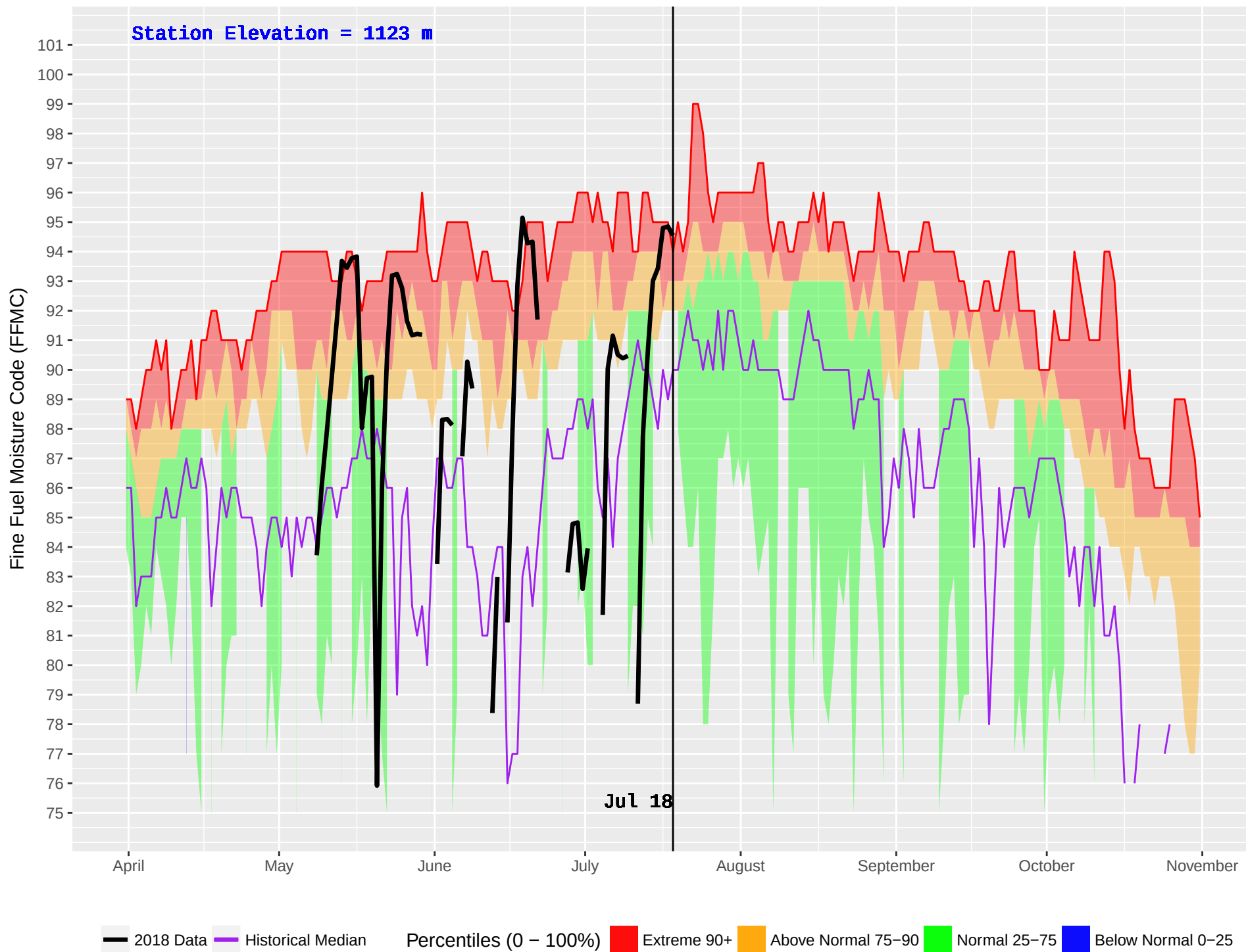
MCLEAN LAKE (311) : Historical (1987–2016) and Current (2018) Daily Fine Fuel Moisture Code (FFMC)
